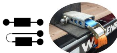
Figure 6. Profile-to-trailer connector
