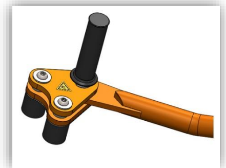
Fig.2 Rotating head with handgrip
